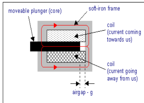
Figure 5.6 – Structure of a Solenoid
