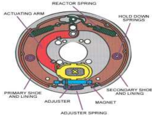
Figure 3.4 – Electromagnetic brake assembly
