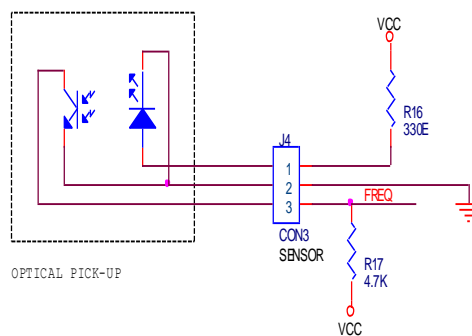
Figure 4.4 – Vehicle speed sensor Circuit
