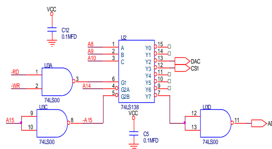
Figure 4.7 – Decoder Circuit
