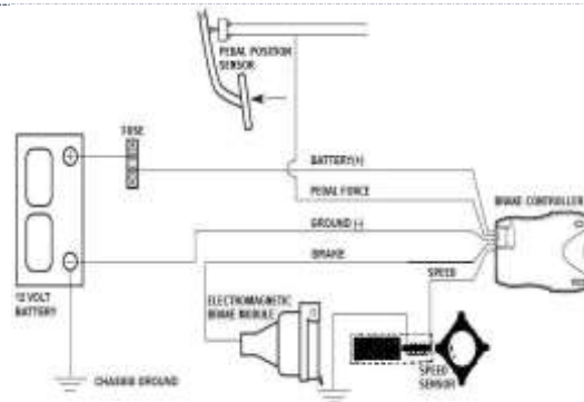
Figure 4.1 – Block Diagram of the System
